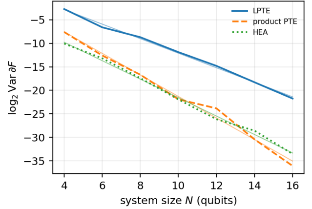
FIG. 7 Noiseless scaling of fidelity-gradient variance versus system size for LPTE (solid), product PTE (dashed), and a hardware-efficient ansatz (dotted), \log_2 scale, ten random initializations per point. Lines are least-squares fits: slopes -1.55 (LPTE), -2.29 (product), -1.96 (HEA).
